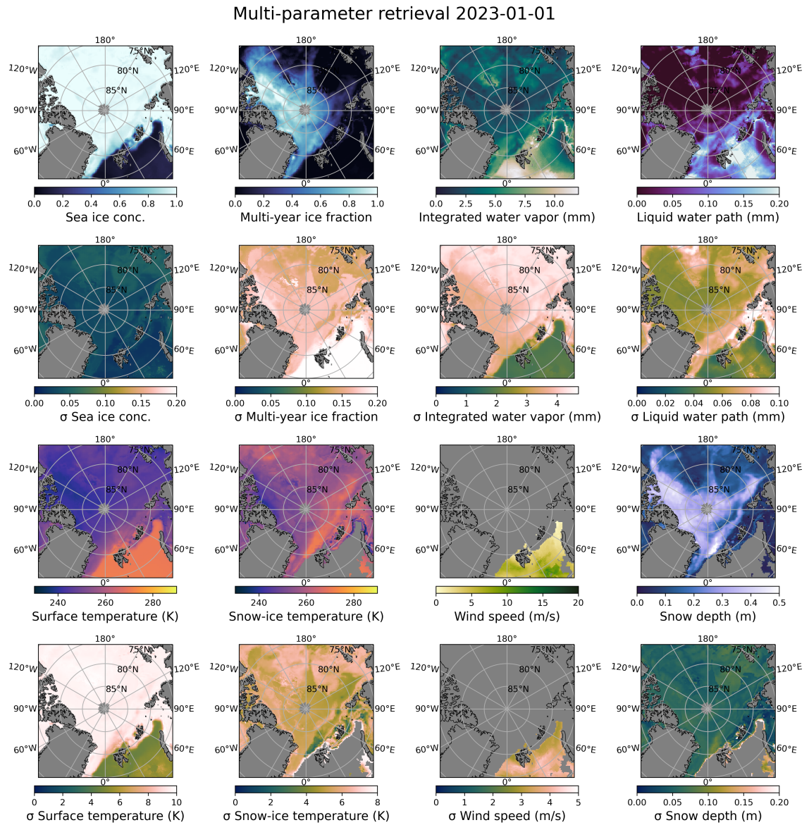
Figure 1: Maps of retrieved parameters and their retrieved uncertainties for January 1, 2023.
